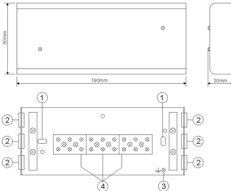
Fig.1. The junction box .
