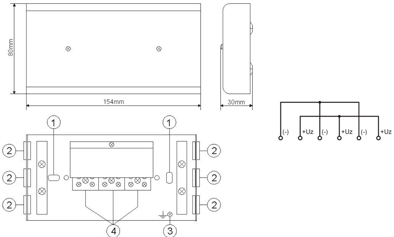
Fig.1. The junction box and wiring diagram.
